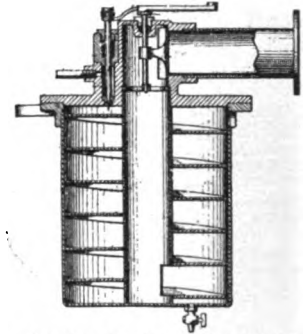
Section Looby Carbureter.
